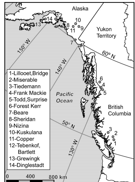
Figure 1. Location of study glaciers in Pacific North America.
