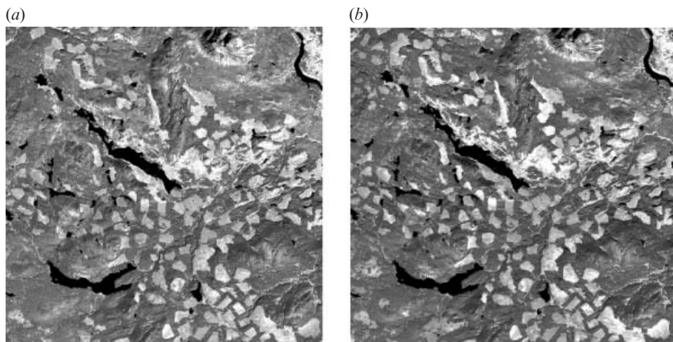
Figure 1. Landsat NIR (band 4; 0.76–0.90 \mu\text{m} ) imagery for (a) 1995 and (b) 2001. Low values represent water, intermediate values represent forest, and high values represent exposed areas.
